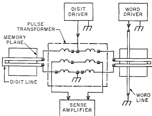
Figure 3—Scheme for eliminating stray signals.
