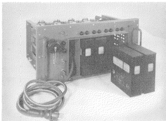
Figure 9—Stabilized battery charger with 2 of 4 batteries in place.
