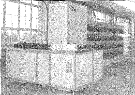
Figure 13—Automatic letter-sorting machine that reads 4-digit code numbers and sorts to 100 destinations.
