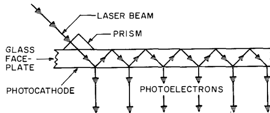
Figure 14—Increased response is obtained by producing multiple reflections of a laser beam within the glass faceplate of a multiplier phototube.
