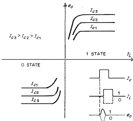
Figure 3—Output characteristics of a magnetic thin-film sample.
