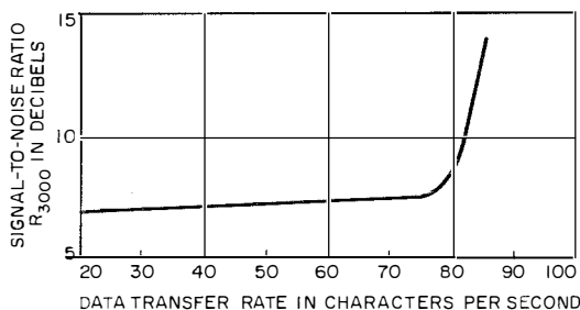
Figure 10—Signal-to-noise ratio as a function of data transfer rate at a character error rate of 10^{-3} and a noise bandwidth of 3000 hertz for GH-4002 with timing channel.
