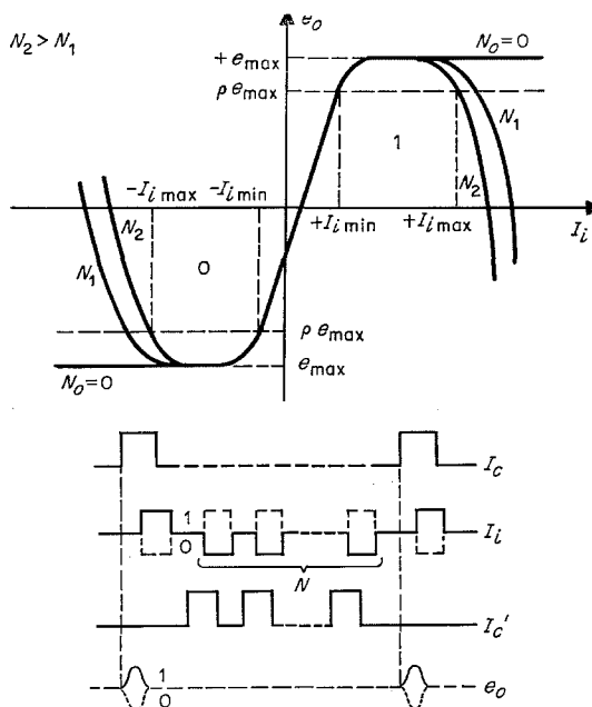
Figure 5—Disturbed output characteristics.
