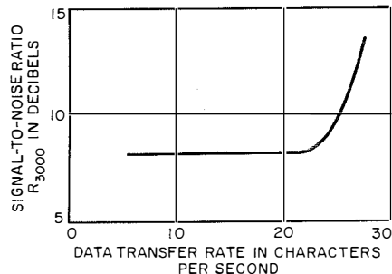
Figure 11—Signal-to-noise ratio as a function of data transfer rate at a character error rate of 10^{-3} and a noise bandwidth of 3000 hertz for GH-4002 without timing channel.
