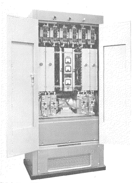
Figure 1—Rear of localizer transmitter. Along the top are 6 reflectometers with 3 meters for them centrally below. The motor for the mechanical modulators is visible just below the meters.
